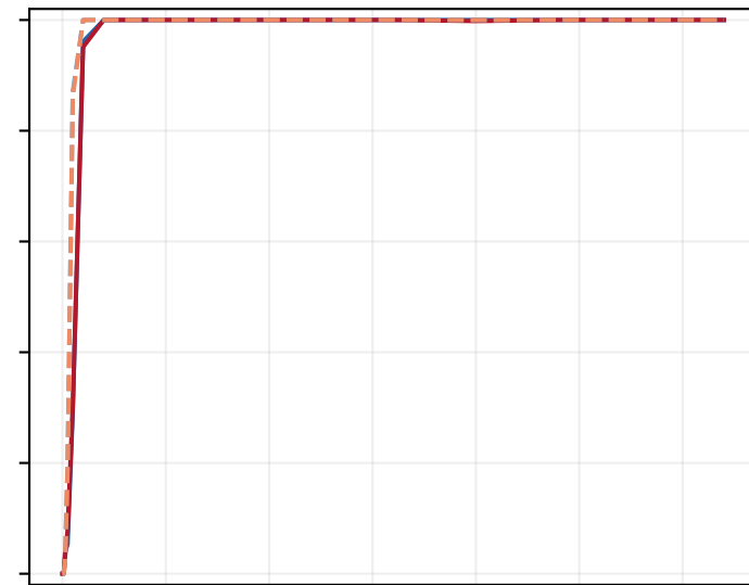
Atomic background
