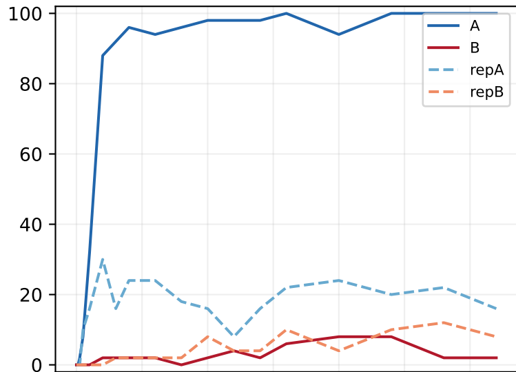
Held-out A→A
