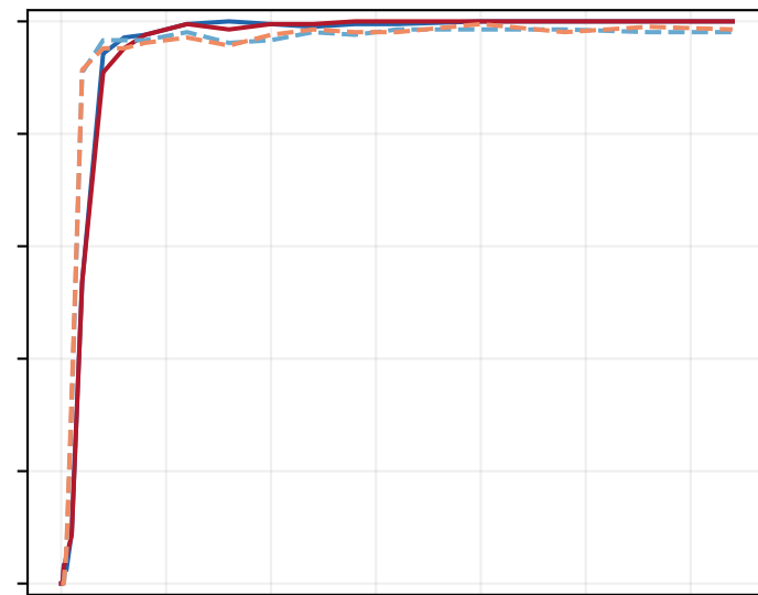
Held-out BG→BG
