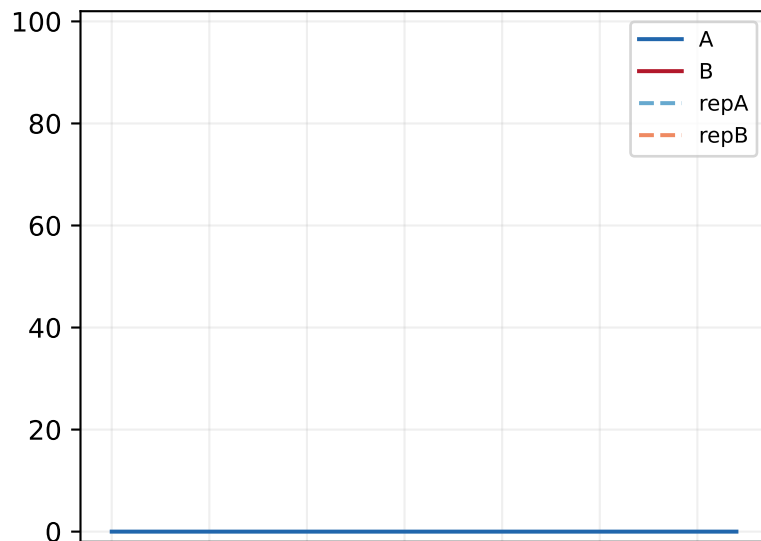
Held-out A→A
