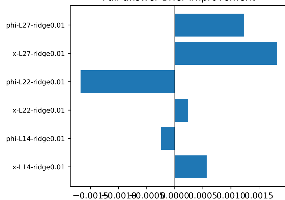
Full-answer Brier improvement
