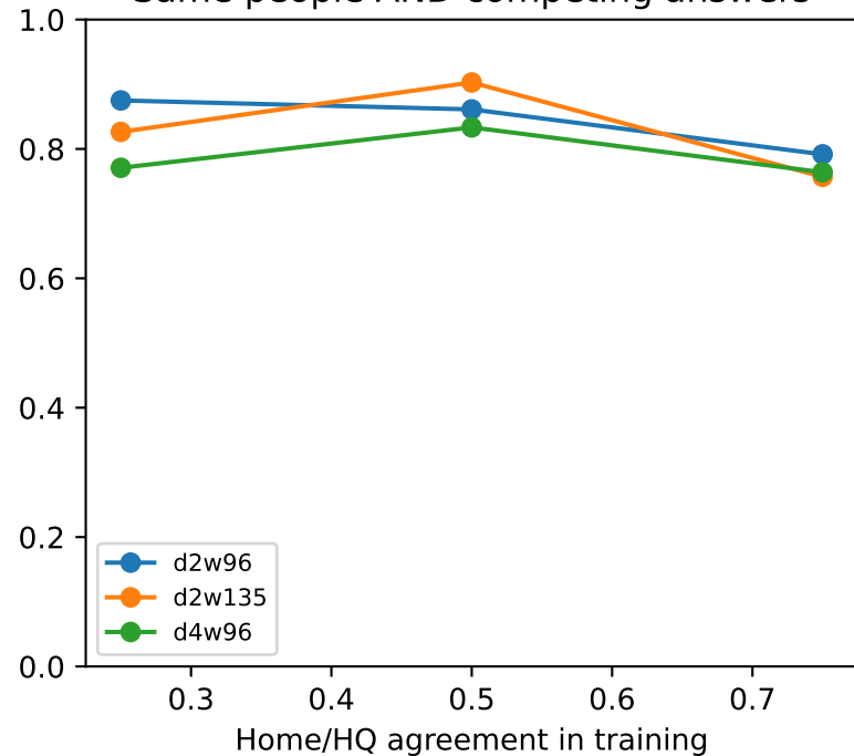
Same people AND competing answers
