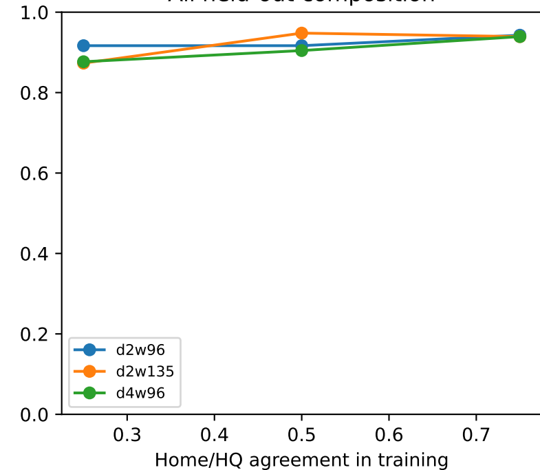
All held-out composition
