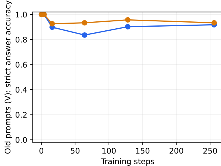
Qwen3-0.6B, layer 14 down updates; 4 development episodes
