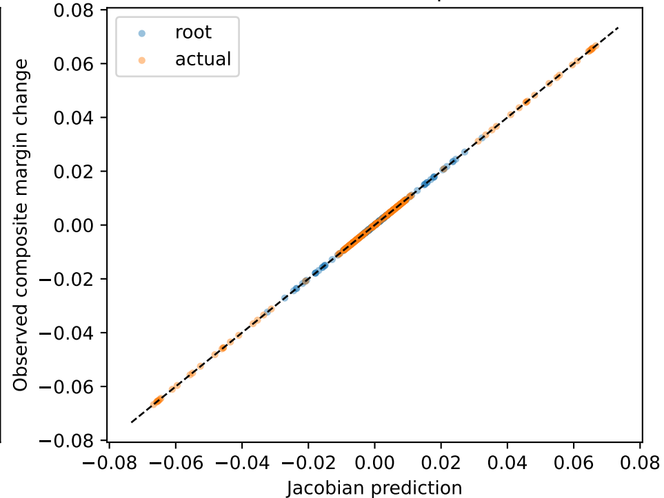
Source-isolated small-step intervention
