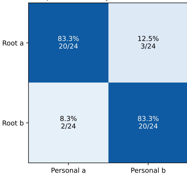
Composite accuracy: four factual states
