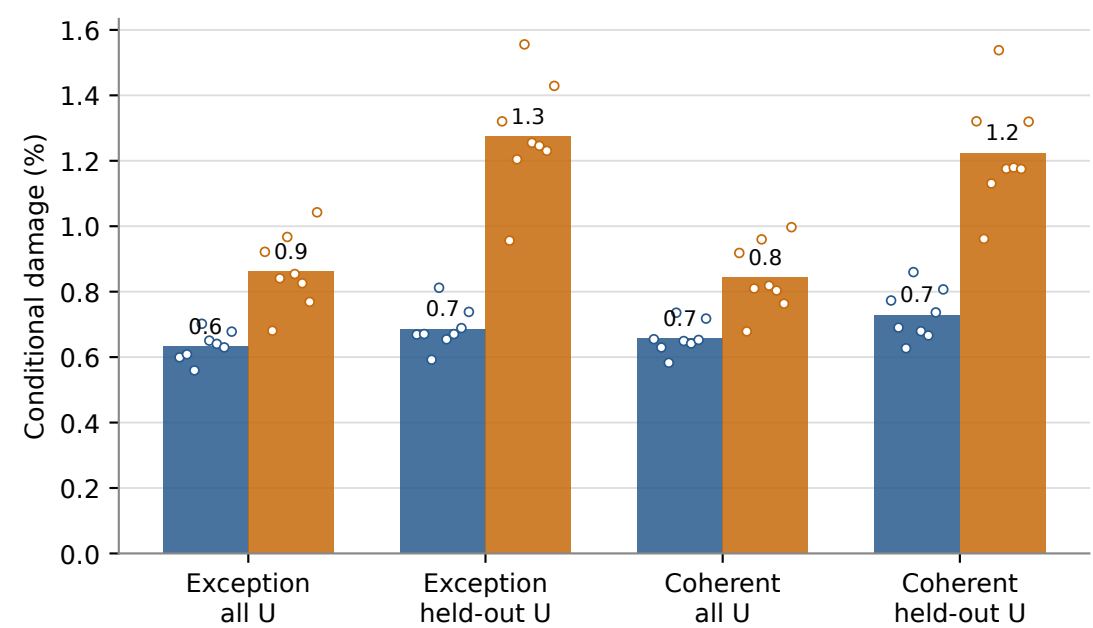
(c) Global damage among previously correct facts
