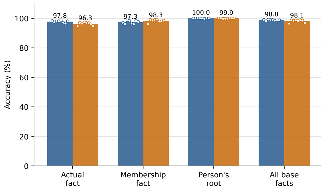
(c) Basic knowledge remains a separate check
