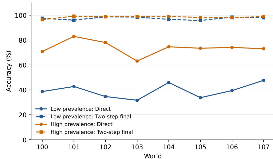
(b) Original exceptions: autonomous two-step
