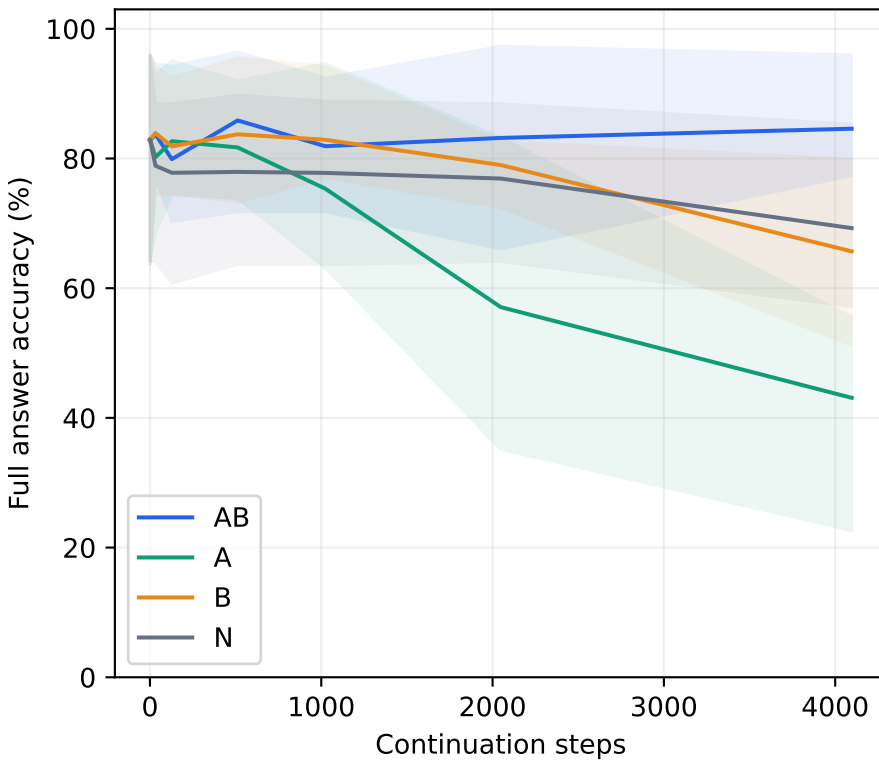
Target held-out composition
