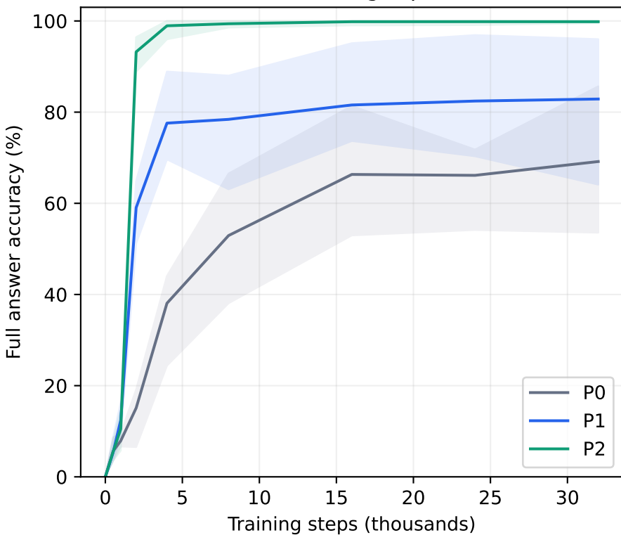
Held-out target paths
