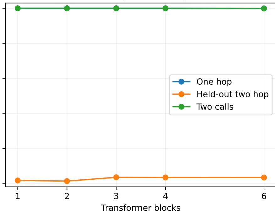
8192 optimizer steps
