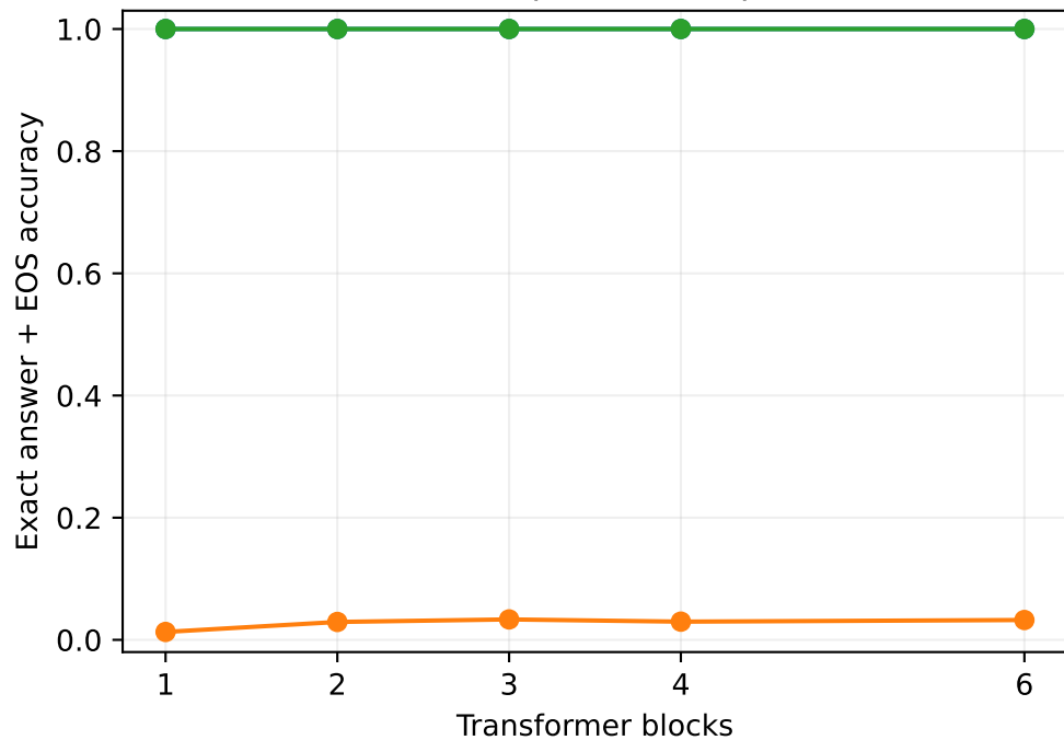
4096 optimizer steps
