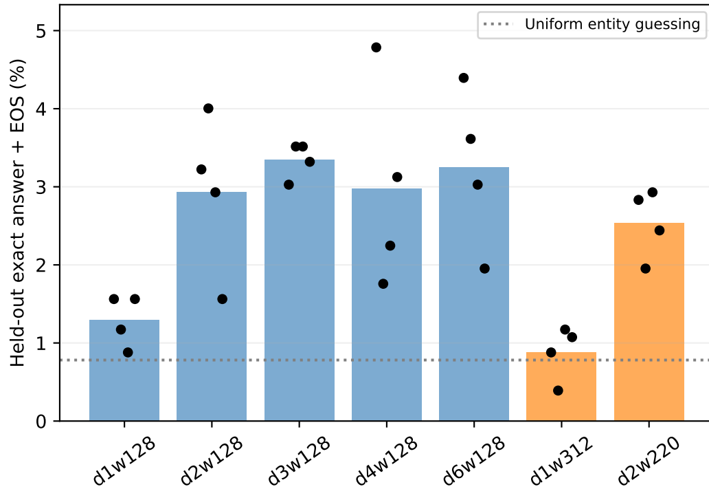
4096 training steps; dots = 2 worlds x 2 seeds
