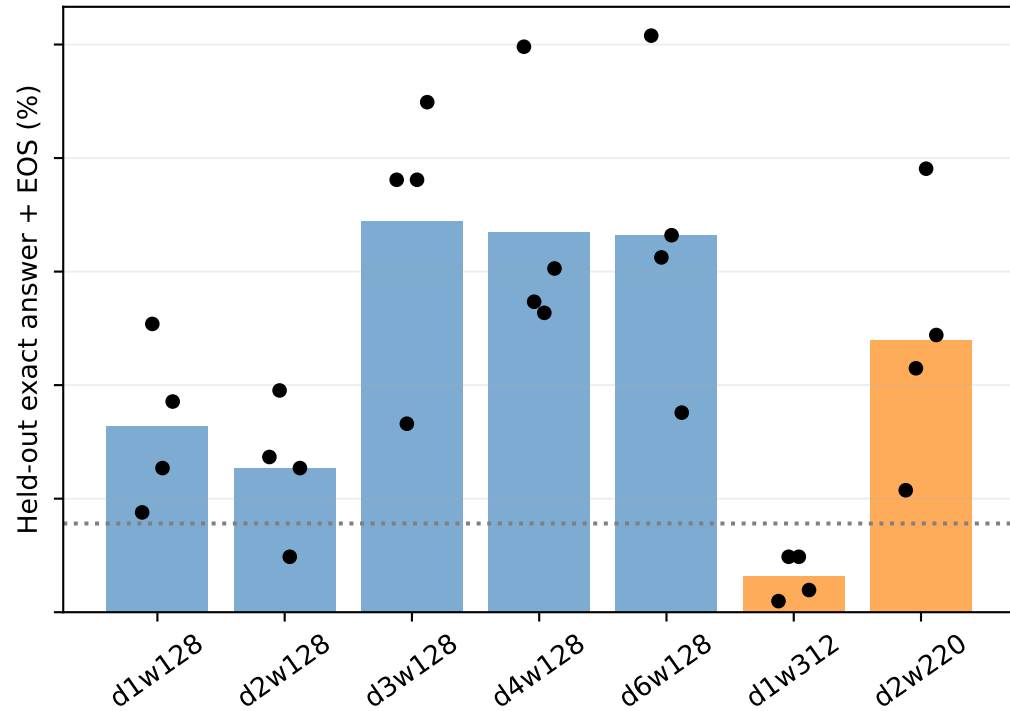
8192 training steps; dots = 2 worlds x 2 seeds
