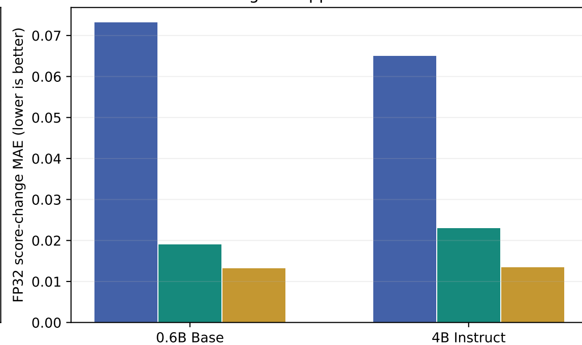
2Wiki: gold-support interventions
