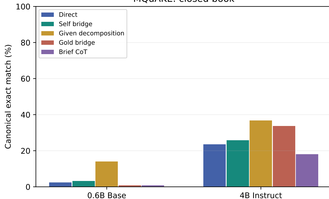
MQuAKE: closed-book interventions
