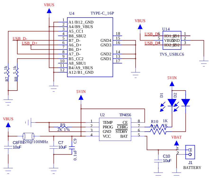
Battery Recharge
