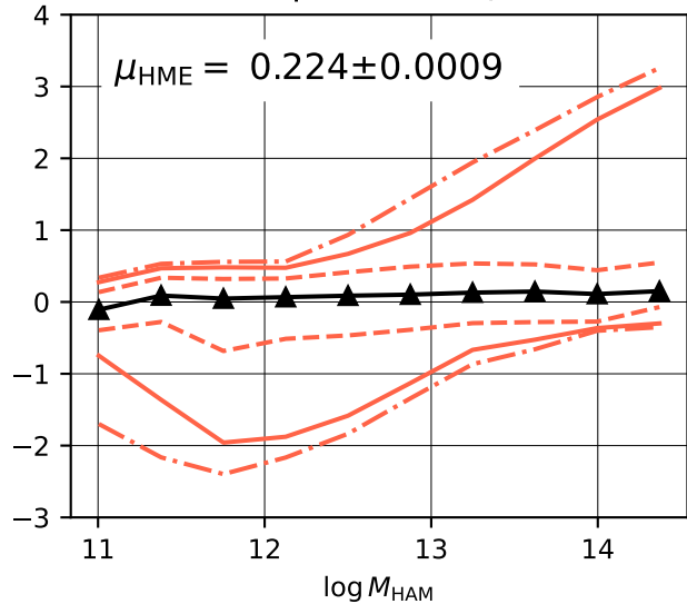
G3 Group Finder ( b_v = 1.2 )
