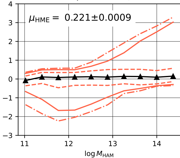
G3 Group Finder ( b_v = 0.8 )
