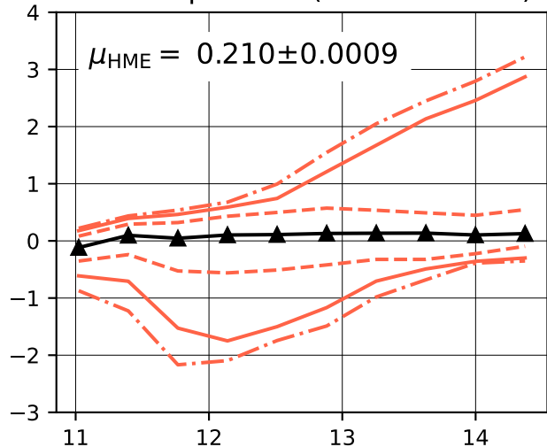
G3 Group Finder ( b_v = 1.2 )
