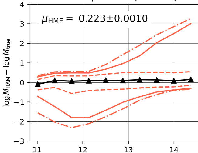
G3 Group Finder ( b_v = 0.8 )
