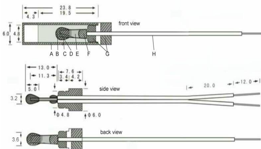
Drawing (unit : mm)
