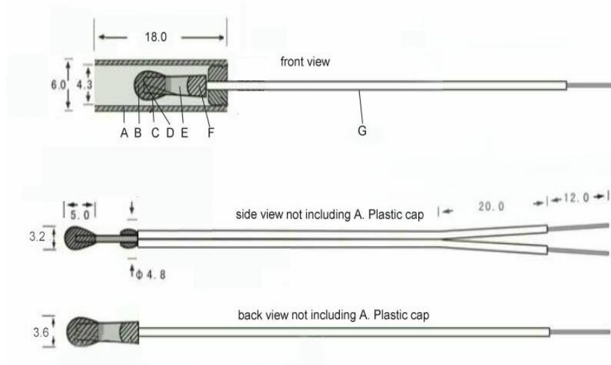
Drawing (unit : mm)
