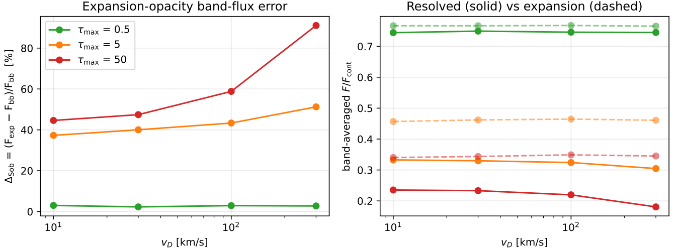
Figure 8. First validity-map slice: \Delta_{\text{exp}} vs Doppler width for three overall line-strength scalings of the La II forest. Right panel: expansion-opacity fluxes (dashed) are blind to v_D , while resolved fluxes (solid) drop as profiles widen.
