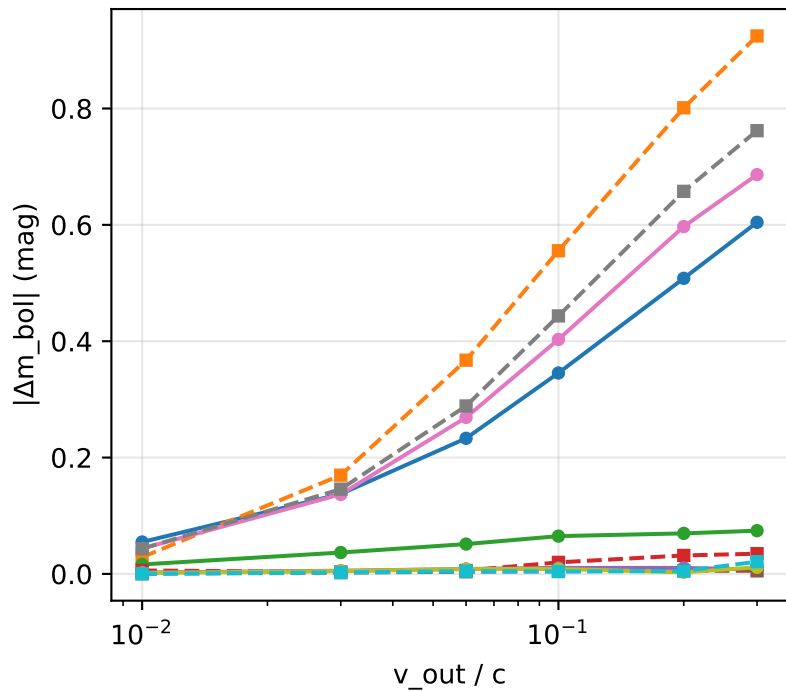
closure error against ejecta velocity (phase 11 velocity scans, top-hat bands)
