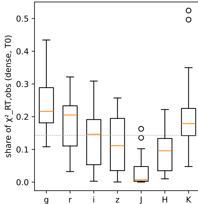
which band carries the \chi^2
