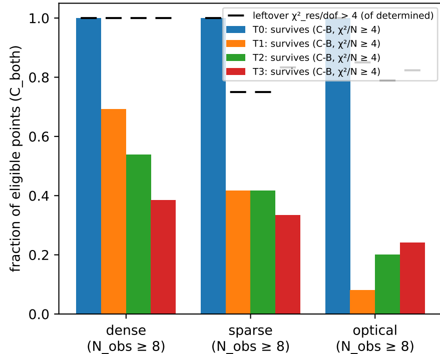
Gate 3 by scenario and tangent space
