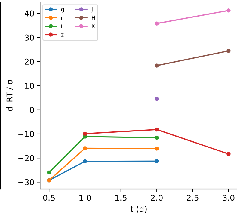
(0.01, 0.1, 0.01), dense: N_{\text{obs}} = 17 , \chi^2/N = 500 , C-B
