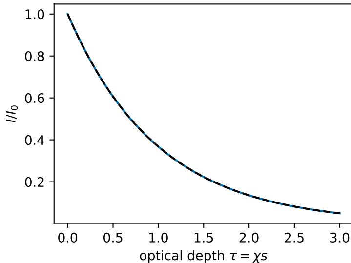
Beer-Lambert: the same curve against distance and against optical depth
