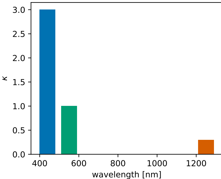
opacity per group
