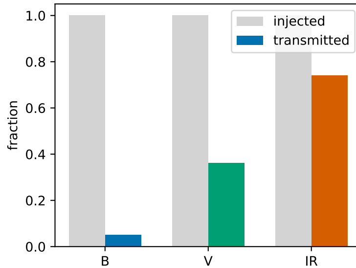
input vs output SED, pure extinction
