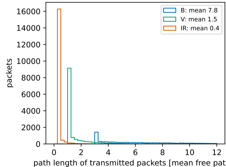
elastic scattering: escape path by group
