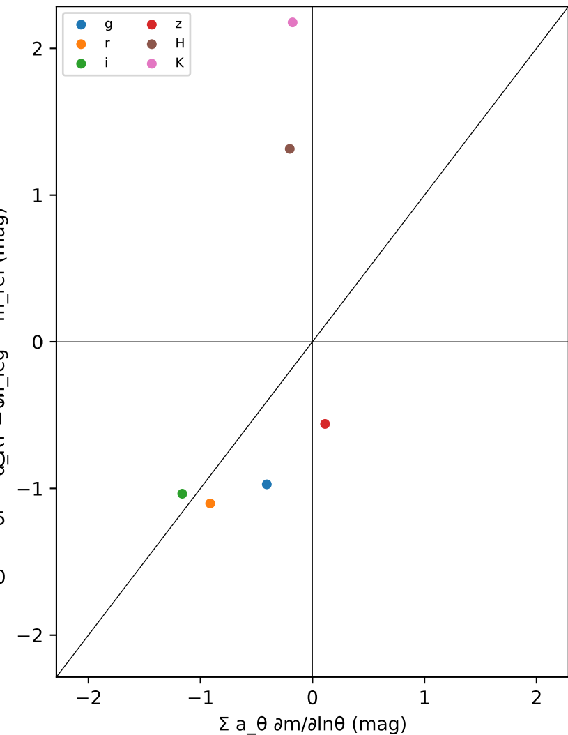
central point, C_both: a = (+0.14, +0.34, -1.83) R = 0.73, \chi^2_{\text{RT}}/N = 344.4 , \chi^2_{\text{res}}/N = 185.6 , class C-B
