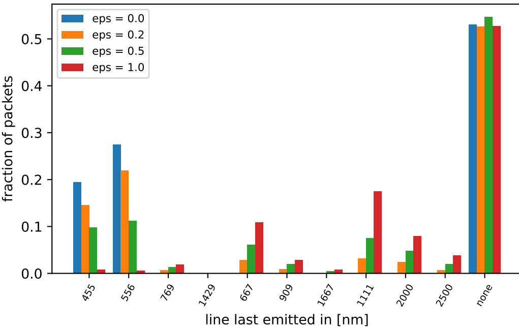
emergent line spectrum of identical blue packets
