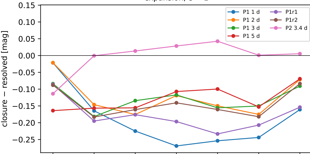
line-binned, \varepsilon = 1
