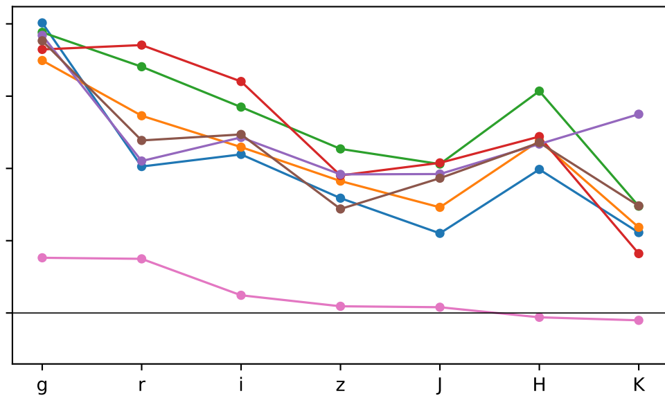
line-binned, fluorescence
