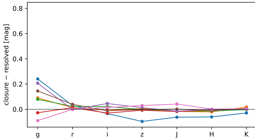
line-binned, \varepsilon = 1
