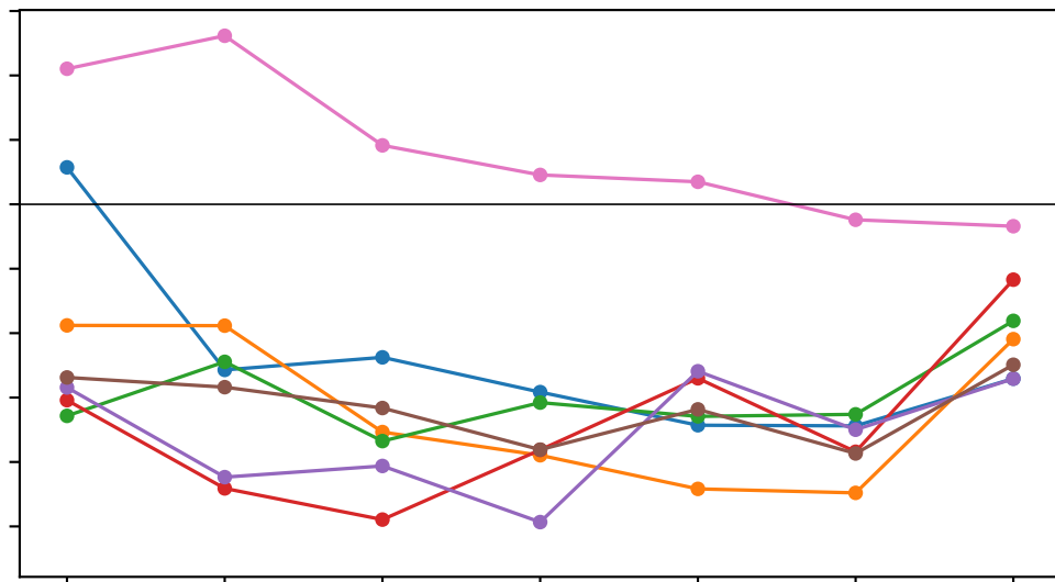
line-binned, fluorescence
