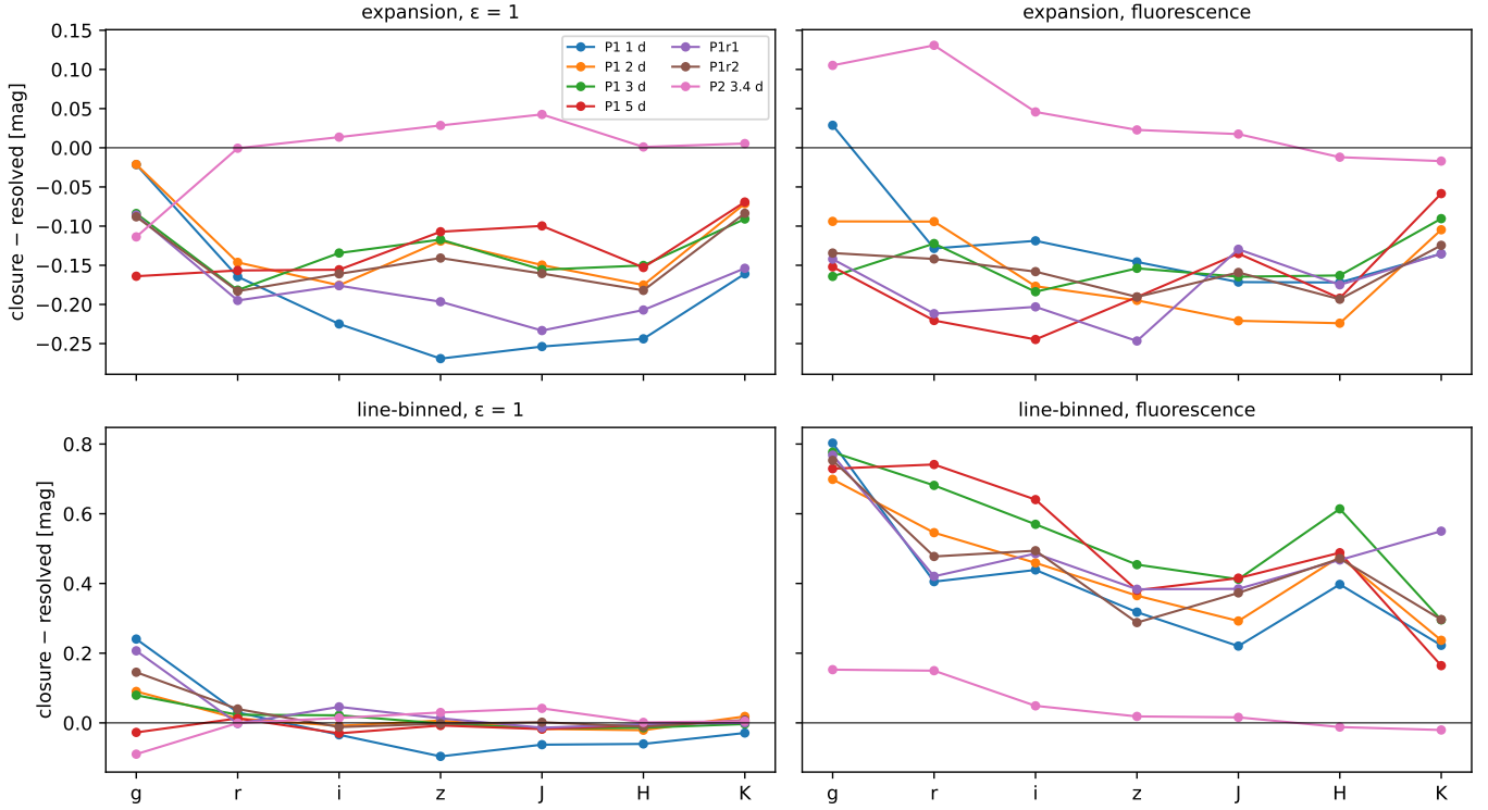
F62: the two closures under complete redistribution and under explicit fluorescence (fixed transport)
