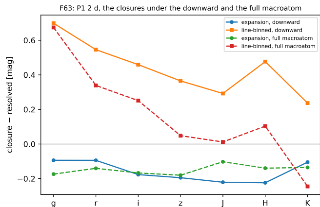
Figure 4. Closure minus resolved transport per band on P1 at 2 d under the downward macroatom (solid) and under the full macroatom with upward transitions driven by an imposed diluted Planck field (dashed), for the expansion (circles) and line-binned (squares) treatments.
