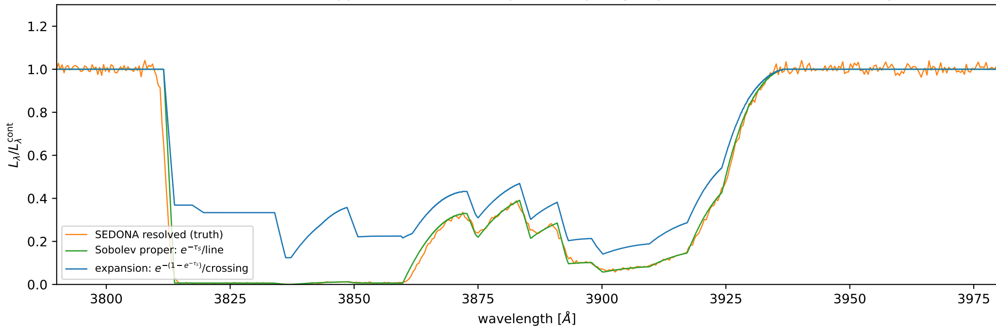
La II forest: the Sobolev approximation vs its expansion-opacity implementation (T = 3000 K, day 1)
