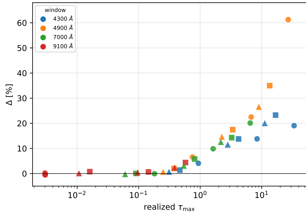
expansion opacity
