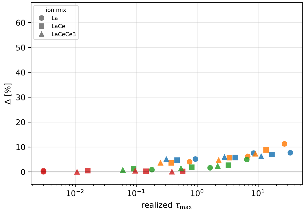
Sobolev proper
