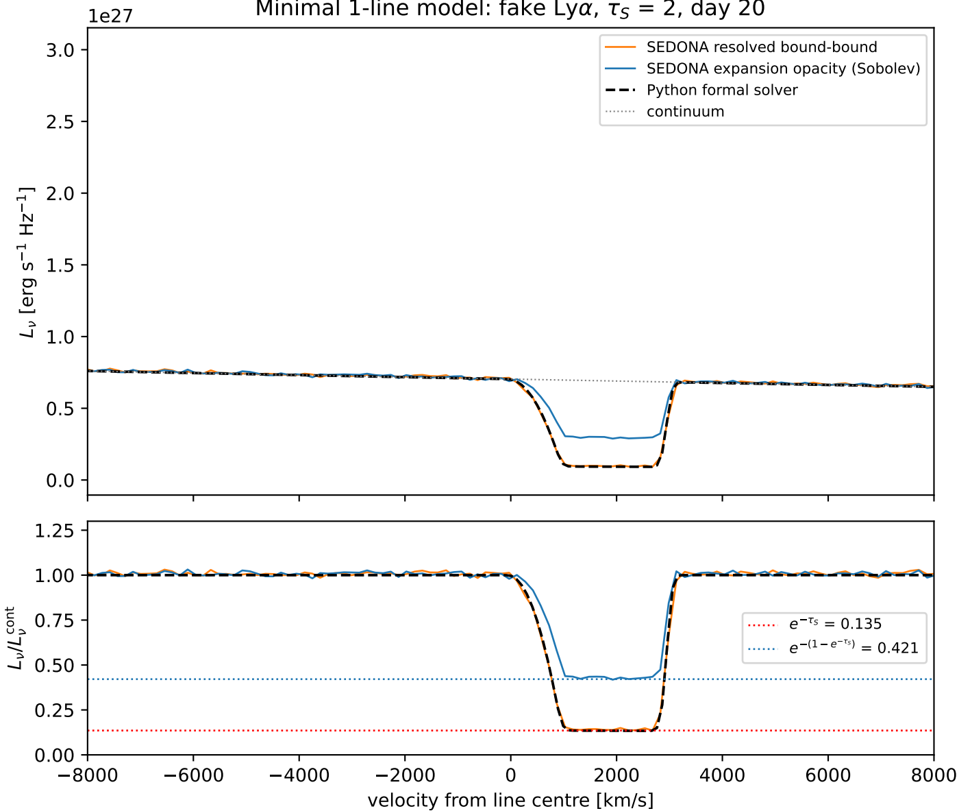
Minimal 1-line model: fake Ly \alpha , \tau_S = 2 , day 20
