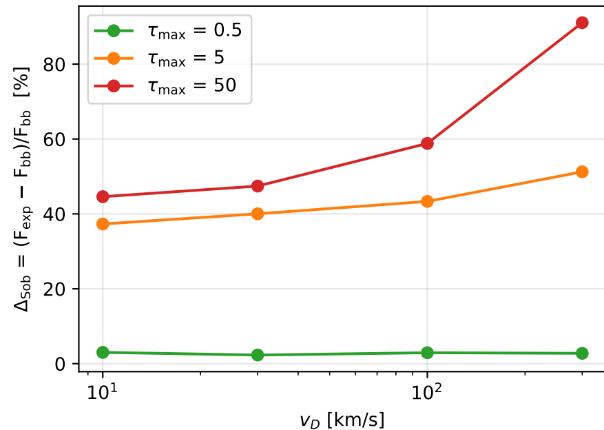
Expansion-opacity band-flux error
