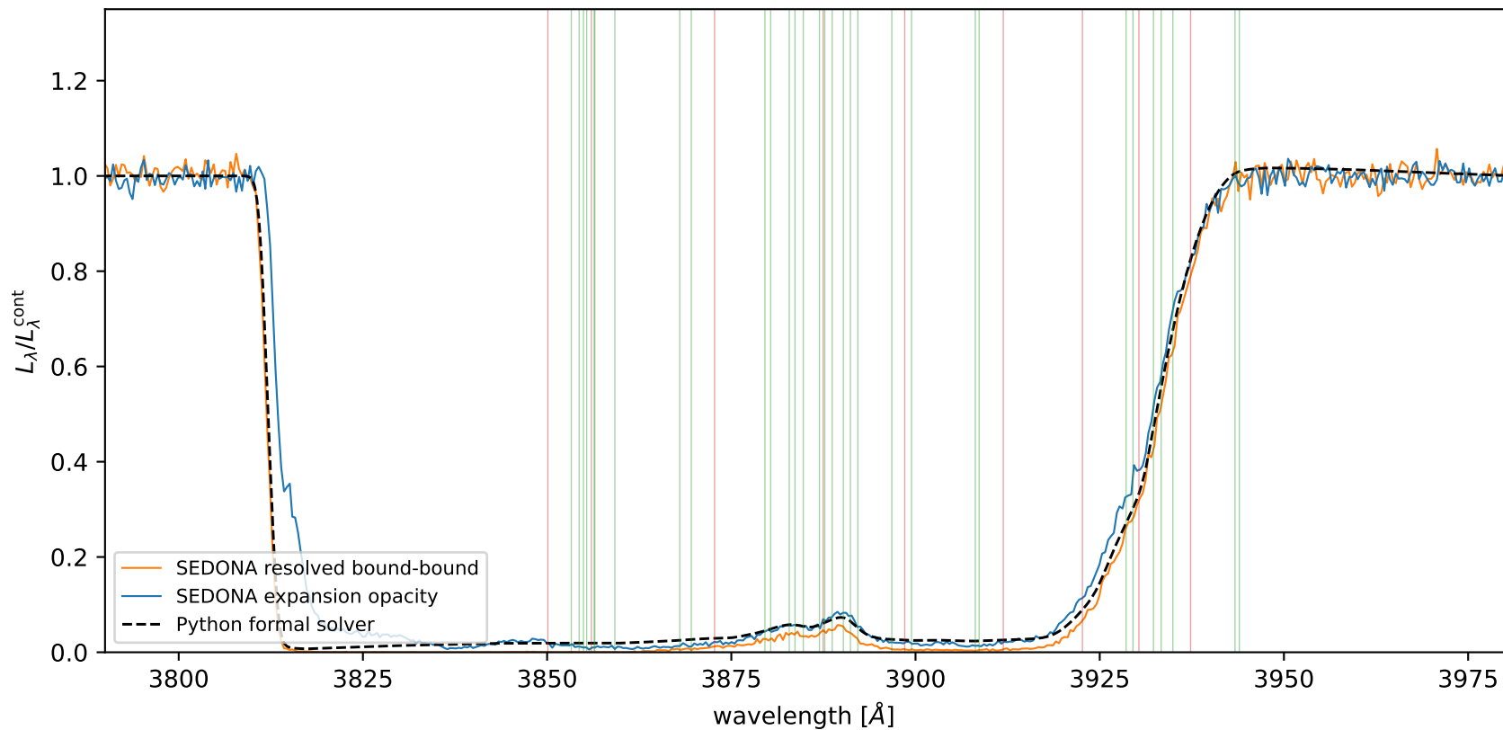
La II + Ce II blend, 3850-3950 Å, T = 3000 K, day 1 (red lines: La II \tau > 0.1 [9]; green: Ce II [31])
