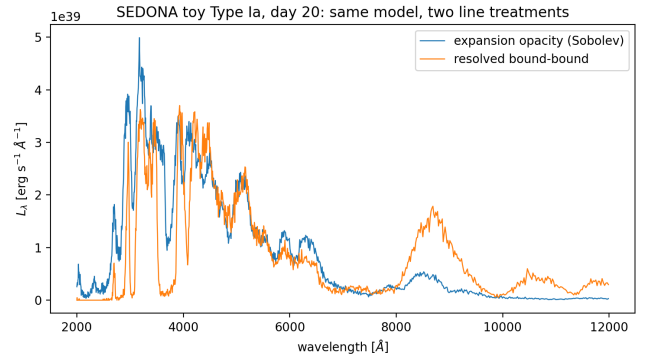
Figure 12. Motivating cost anecdote from a standard SEDONA Type Ia supernova example: the same model runs in 14 s with expansion opacity and 88 min resolved (378×), while redistributing flux from the UV to the near-IR.
