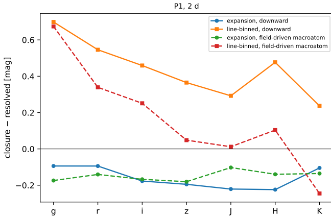
Figure 5. Closure minus resolved transport per band on P1 at 2 d under the downward macroatom (solid) and under the radiation-field-driven macroatom with upward transitions under an imposed diluted Planck field (dashed), for the expansion (circles) and line-binned (squares) treatments.
