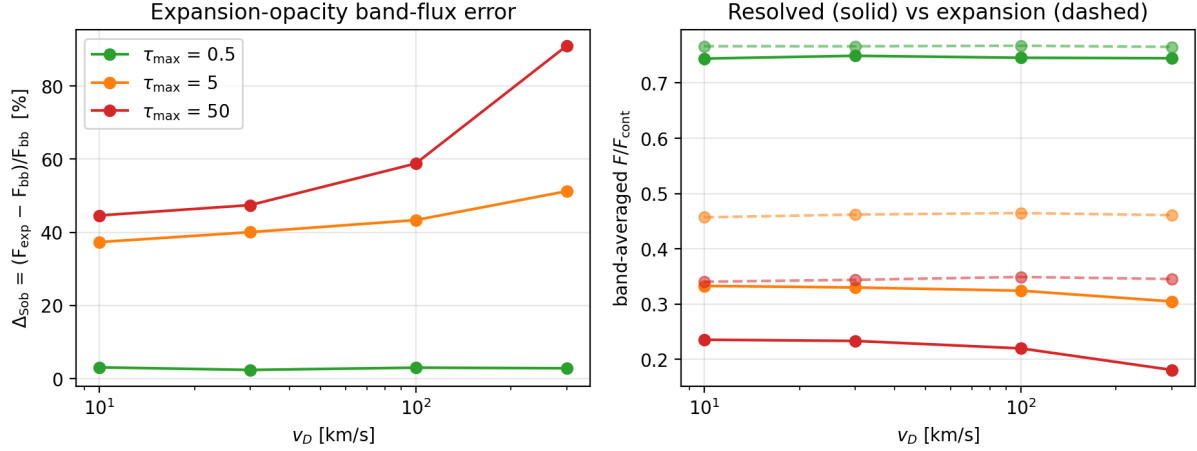
Figure 7: First validity-map slice: \Delta_{\text{Sob}} vs Doppler width for three overall line-strength scalings of the La II forest. Right panel: expansion-opacity fluxes (dashed) are blind to v_D , while resolved fluxes (solid) drop as profiles widen.
