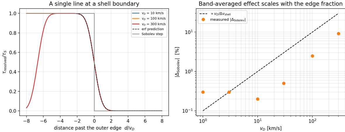
Figure 12: Left: a single line’s resolved optical depth as its resonance is walked out through the outer edge of the line-forming region, in units of the Doppler width. The curves for v_D = 10 , 100 and 300 \text{km s}^{-1} coincide — the effect is self-similar in d/v_D — and follow the error-function prediction exactly, against the hard step that Sobolev applies. The 300 \text{km s}^{-1} curve departs from unity on the left because the shell is then only \sim 7 Doppler widths wide and the inner edge clips as well. Right: the band-averaged consequence tracks v_D/\Delta v_{\text{shell}} .
