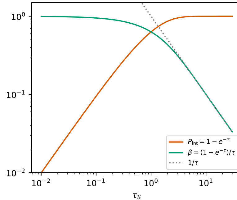
two different quantities called Sobolev
