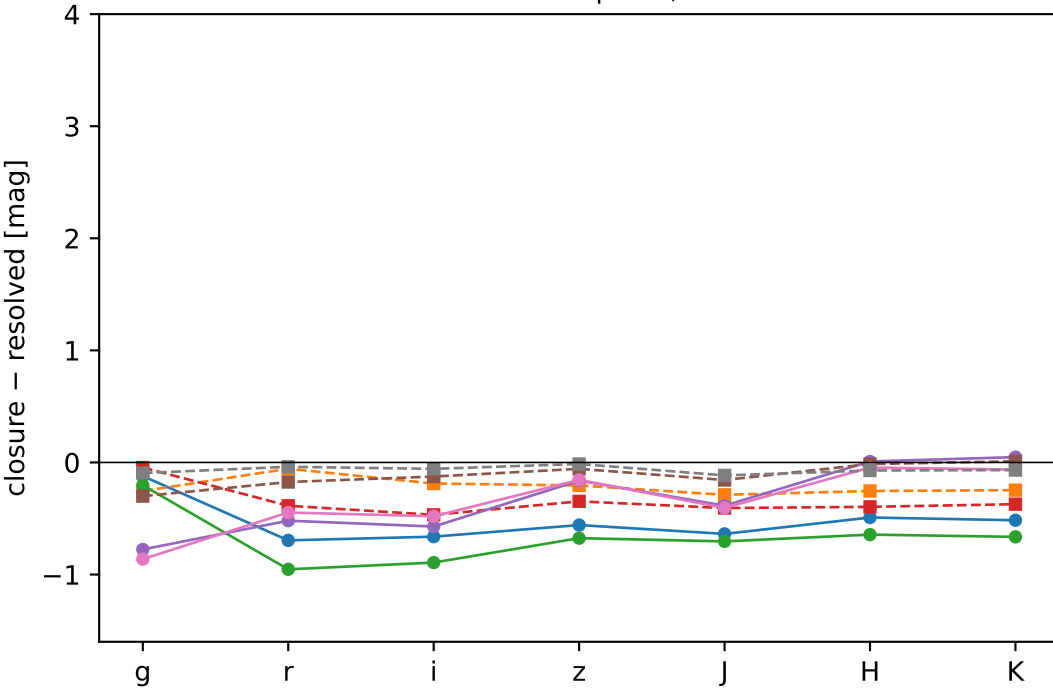
Fontes 4 d snapshot, \varepsilon = 1
