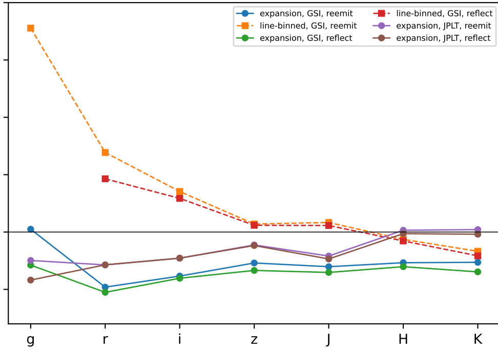
Fontes 4 d snapshot, fluorescence
