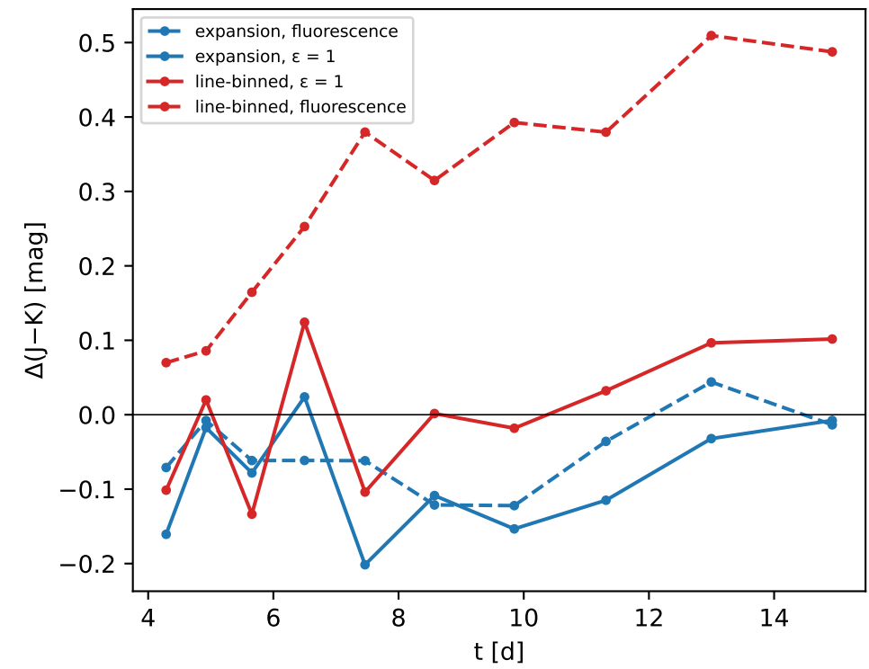
colour residual
