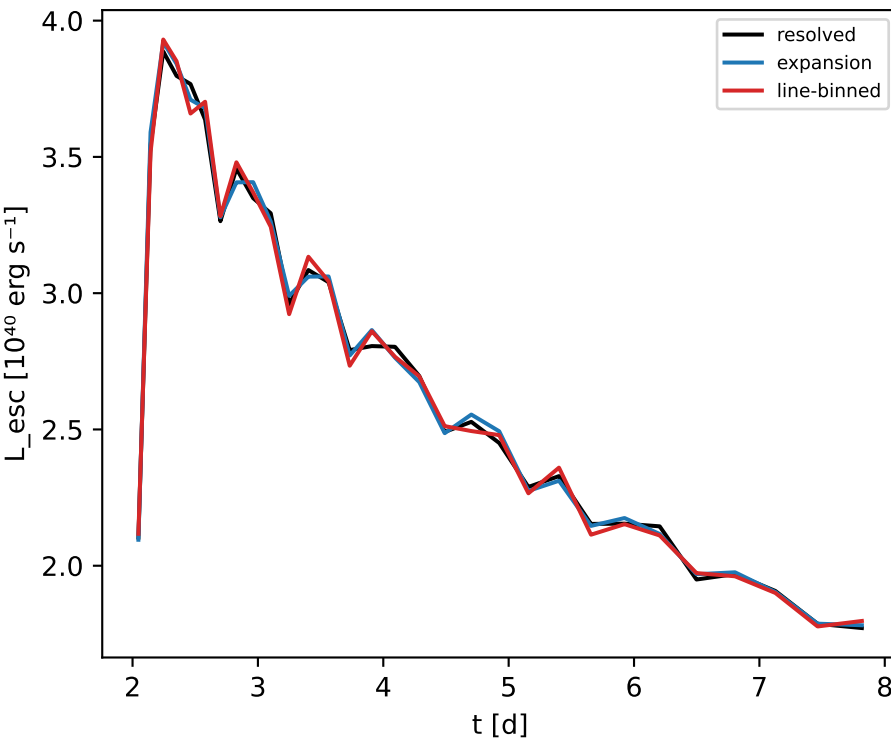
P1-xkn: bolometric, fluorescence
