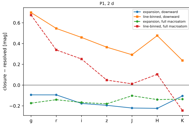
Figure 5. Closure minus resolved transport per band on P1 at 2 d under the downward macroatom (solid) and under the full macroatom with upward transitions driven by an imposed diluted Planck field (dashed), for the expansion (circles) and line-binned (squares) treatments.
