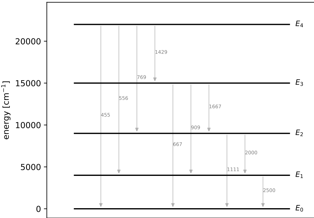
the five-level toy atom and its ten lines [nm]
