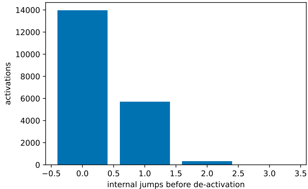
mean 0.32 jumps
