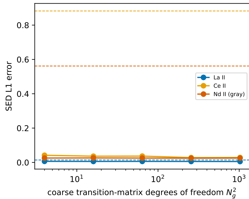
SED error (dashed: \epsilon^* )
