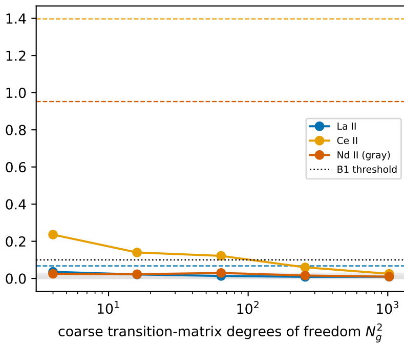
band error (dashed: \epsilon^* )
