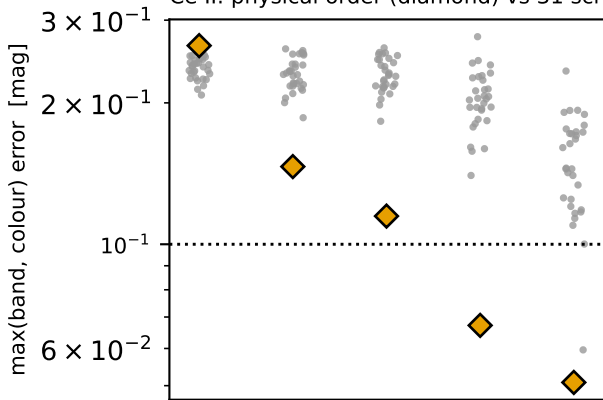
Ce II: physical order (diamond) vs 31 scrambled
