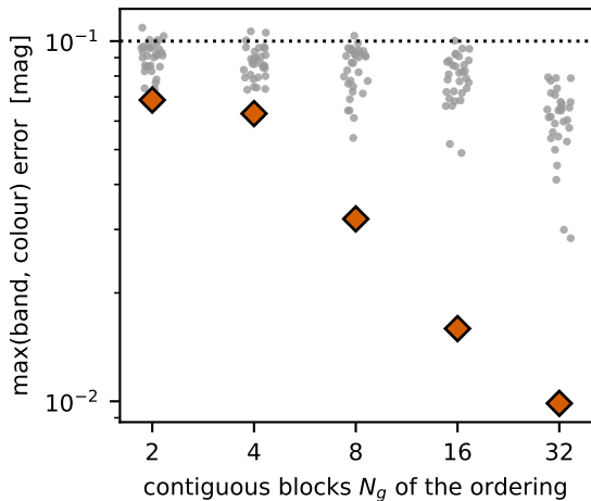
Nd II: physical order (diamond) vs 31 scrambled
