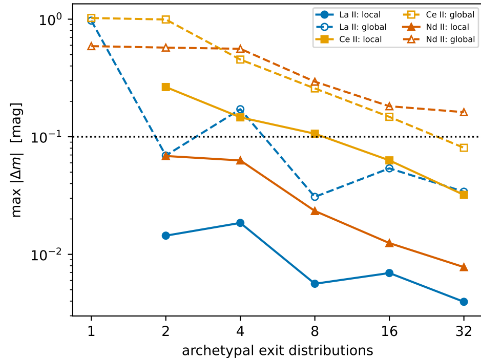
a. transport error (solid: local, open: global)
