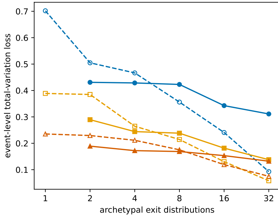
b. microscopic error: the global family wins
