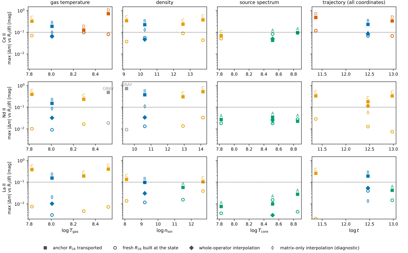
FIG. 2. Transfer is not compression. Maximum photometric error against the state’s own reference for the original operator transported unchanged (filled squares), the operator rebuilt at the state (open circles), and at each axis’ interior point the whole-operator interpolant from the two bracketing states (filled diamonds; matrix-only interpolant, open diamonds). Rows: Ce II, Nd II, the La II control; columns: gas temperature, density, source spectrum, and the trajectory along which all move together. Dotted: the band criterion; the letter is the preregistered reading of each state (A transported operator passes; B only the interpolant; C only a fresh fit; D none at 16 groups). The criterion also bounds the colour error, so a circle below the line can read D. Grey: states excluded by the preregistered validity checks.
