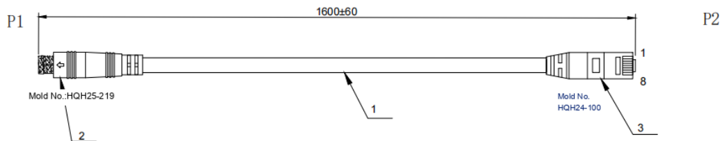
AI Camera Cable
