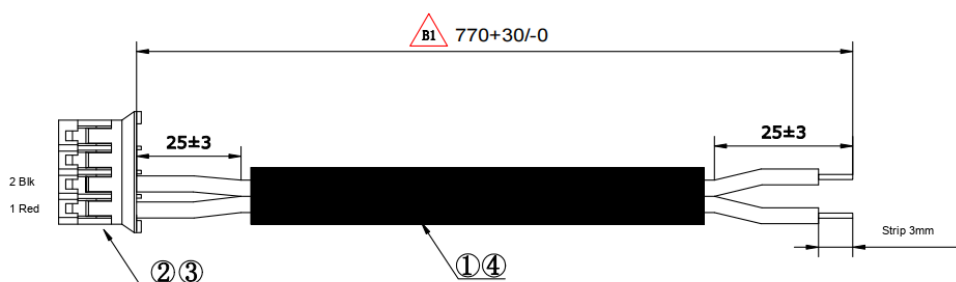
Speaker Cable
