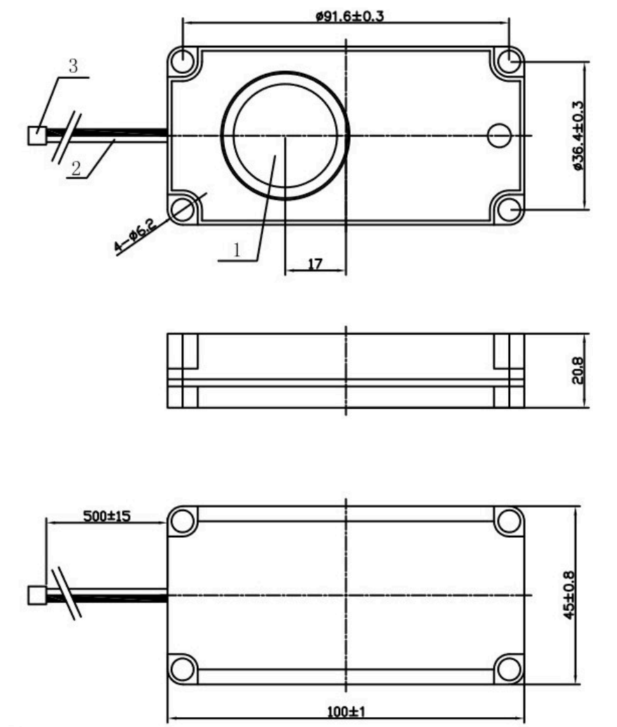
Speaker
