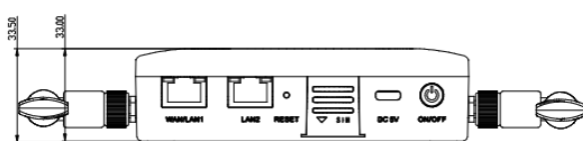
Interface Dimensions
