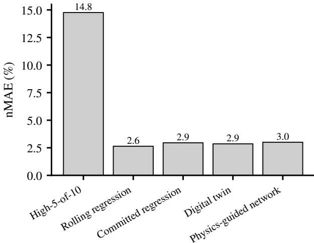
(a) Placebo accuracy
