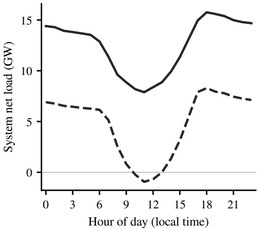
(a) Synthetic 2030 net load
