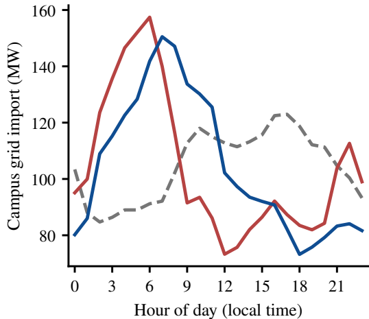
(b) Campus import, summer
