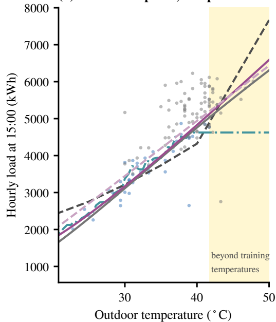
(b) Learned response, Tempe chilled-water meter
