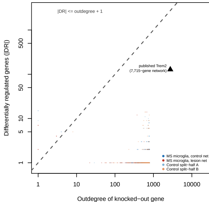
A |DR| is governed by outdegree
